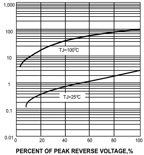
FIG. 4-TYPICAL REVERSE CHARACTERISTICS
