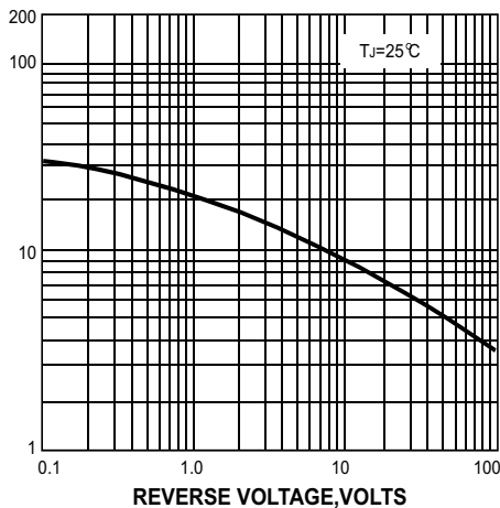
FIG. 5-TYPICAL JUNCTION CAPACITANCE
