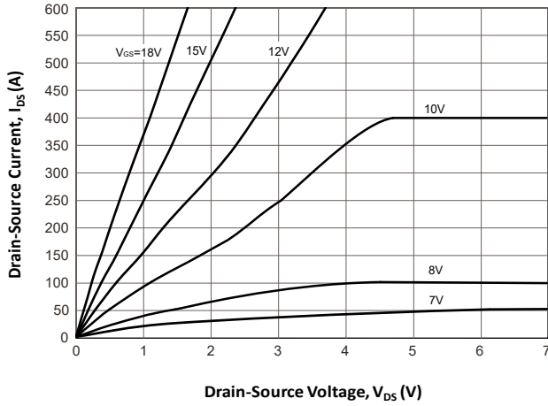
Fig.1 Output Characteristics at T_J = 25^\circ\text{C}
