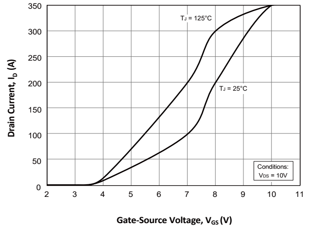
Fig.4 Transfer Characteristics
