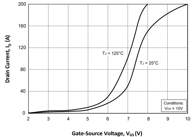
Fig.4 Transfer Characteristics
