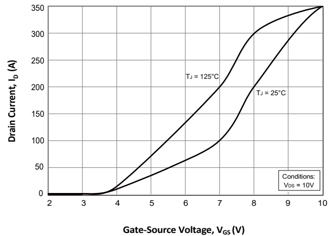
Fig.4 Transfer Characteristics
