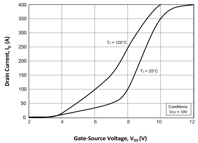
Fig.4 Transfer Characteristics
