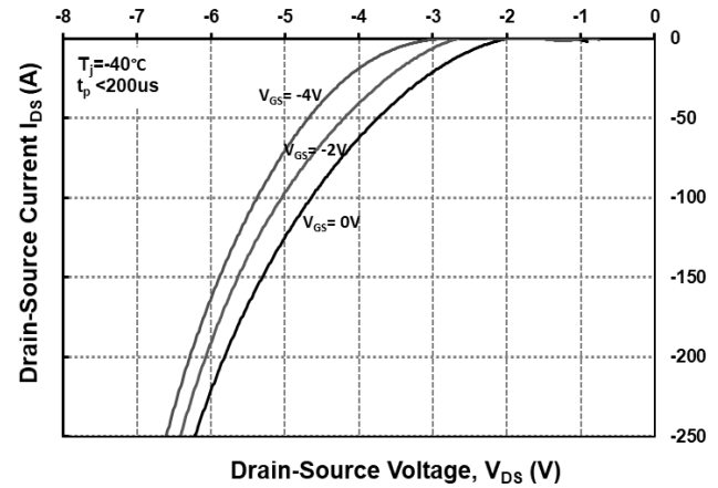
Fig 8. Body Diode Characteristics @ -40^\circ\text{C}
