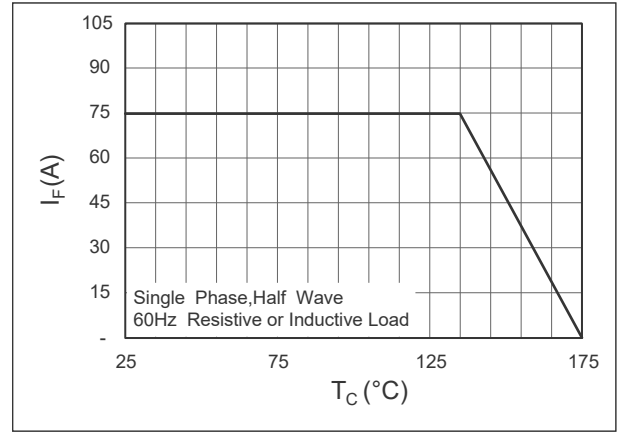
Current Derating
